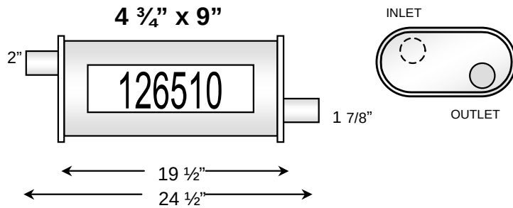
Isuzu Rodeo 96-97, 6 cyl. (3.2L) Four Wheel Drive
