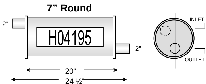
Isuzu Pickup 91-1995, 4 cyl. (2.3L)
