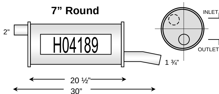
Toyota Previa, 91-1996 4 cyl. (2.4L)
